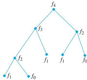
FIGURE 1 Evaluating f_4 Recursively.
